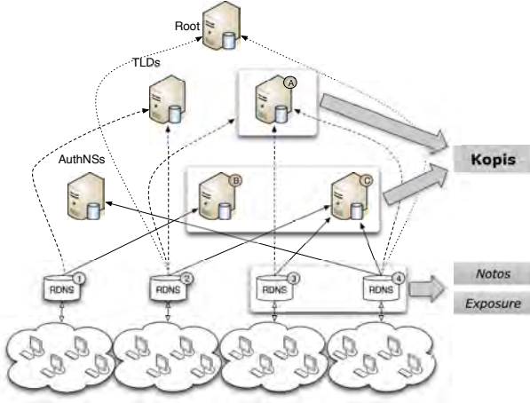
Figure 1: Overview of the levels at which Kopis, Notos, and Exposure perform DNS monitoring.
